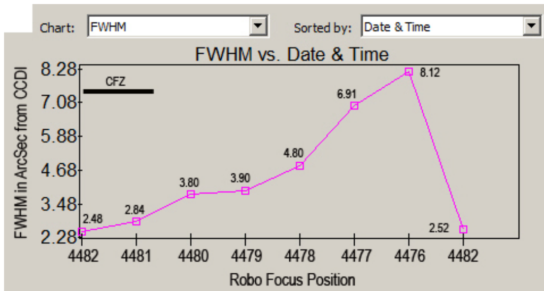
Figure 4. Average FWHM analysis of images shown in Fig. 1 using the green filter.
